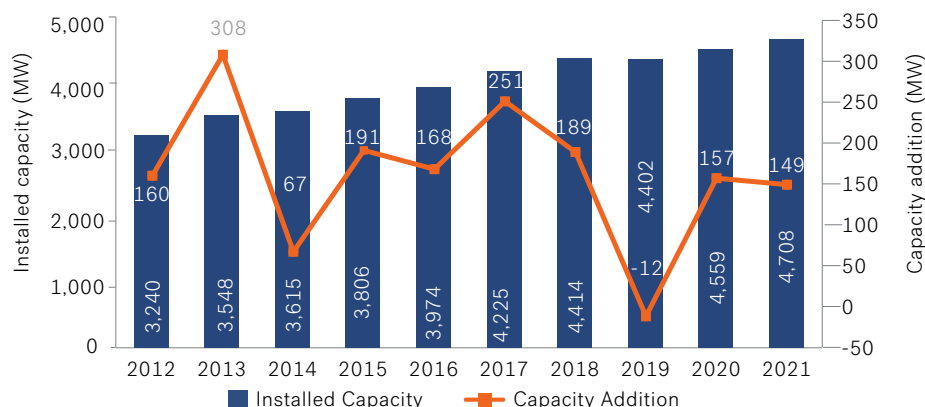
Trend in Installed Onshore Wind Capacity
