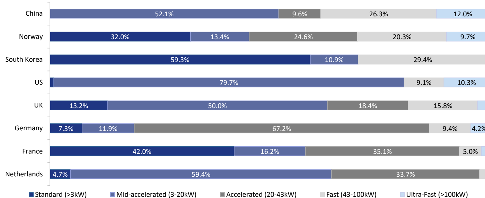
Share of Public EV Charging by Speed, in Select Countries
